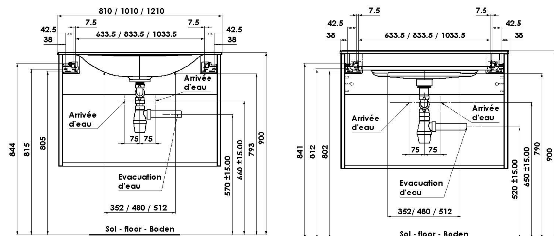
Montage vasque solid surface Installation s/Montage vasque solid surface Installation solid
