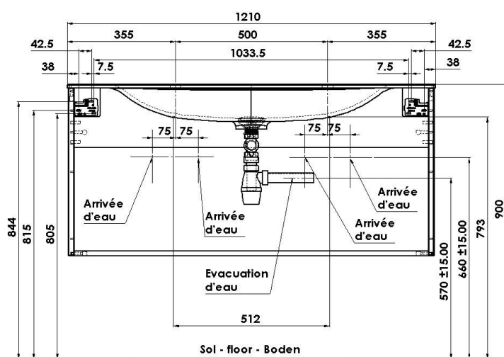
Montage vasque solid surface Installation s/Montage vasque solid surface Installation solid
