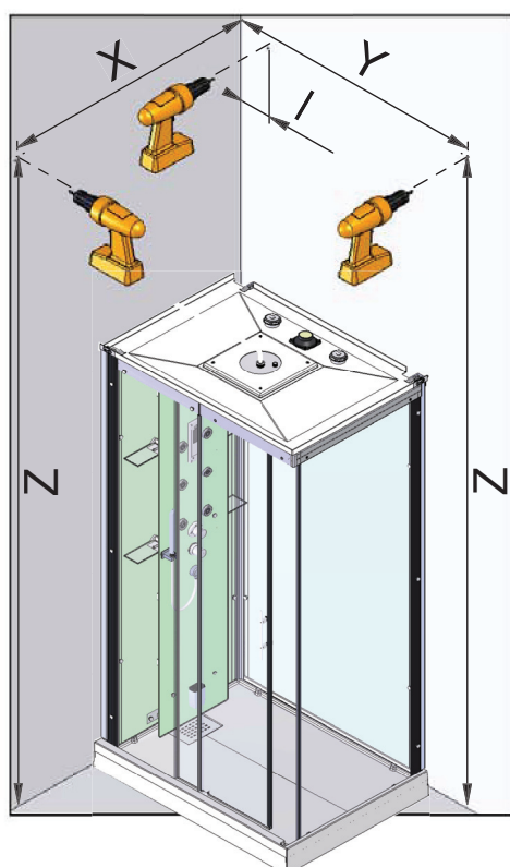
Cabine 110x80
