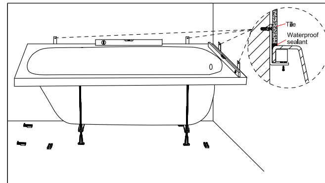
13: Place the bath back into position, fix the wall brackets on the walls and use the waterproof sealant between the bath and tiles.
